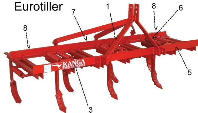
Chisel Plough
